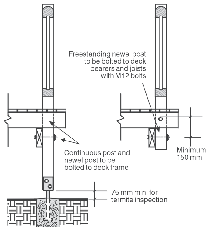
Figure 6. Post and Newel Post Connections
